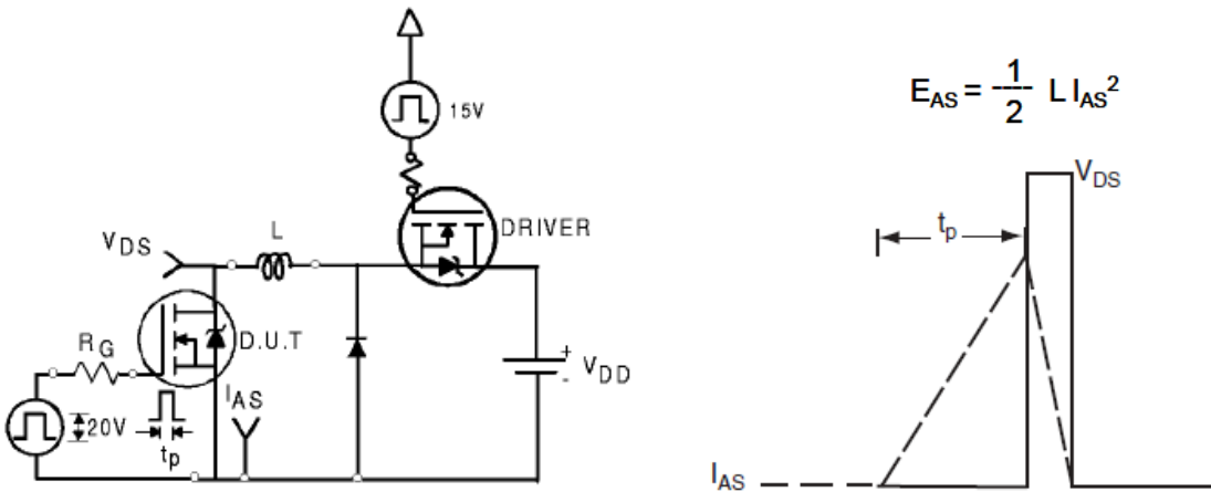
Fig. 21. Unclamped Inductive switching test circuit & waveform
